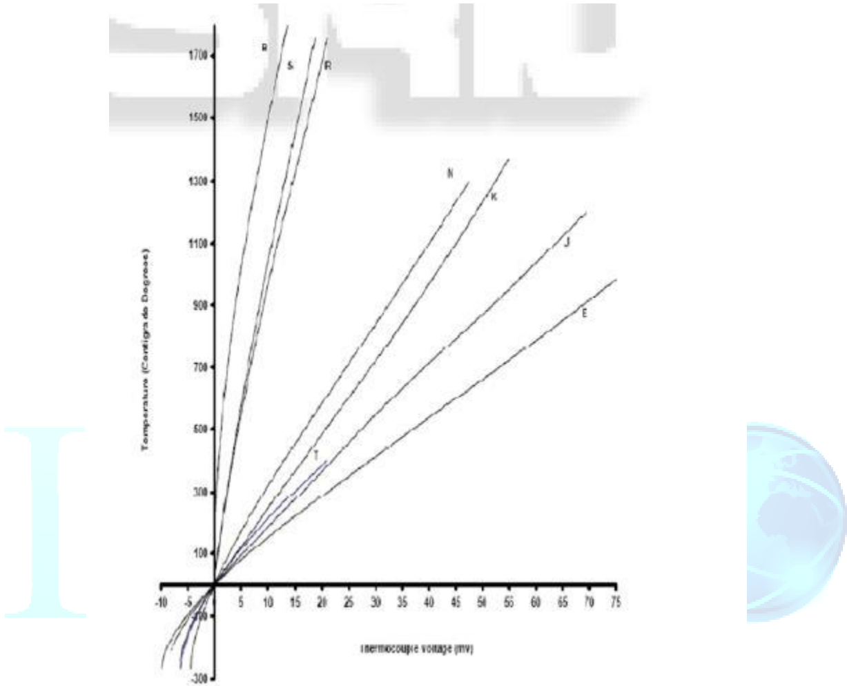
Fig. 4 Voltage-Temperature Characteristics of B, E, J, K, N, R, S, and T Type Thermocouples
