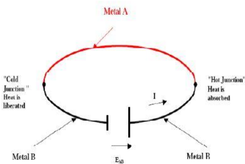
Fig. 2 Illustration of Pelletier Effect
