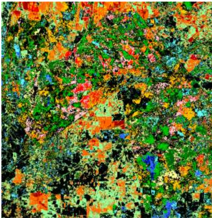
Figure 3: Change Map
