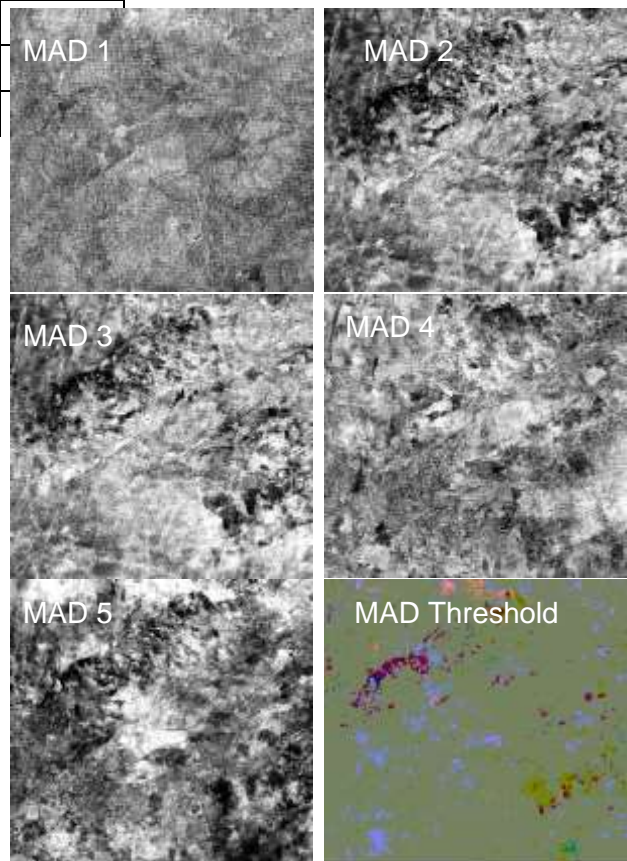
Figure 4: MAD components (1-5) and RGB view of MADs 3, 4, 5 with thresholds.
